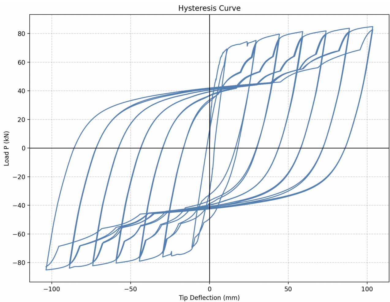
Figure 12. Numerical Response of Model 0 With Force-based elements
