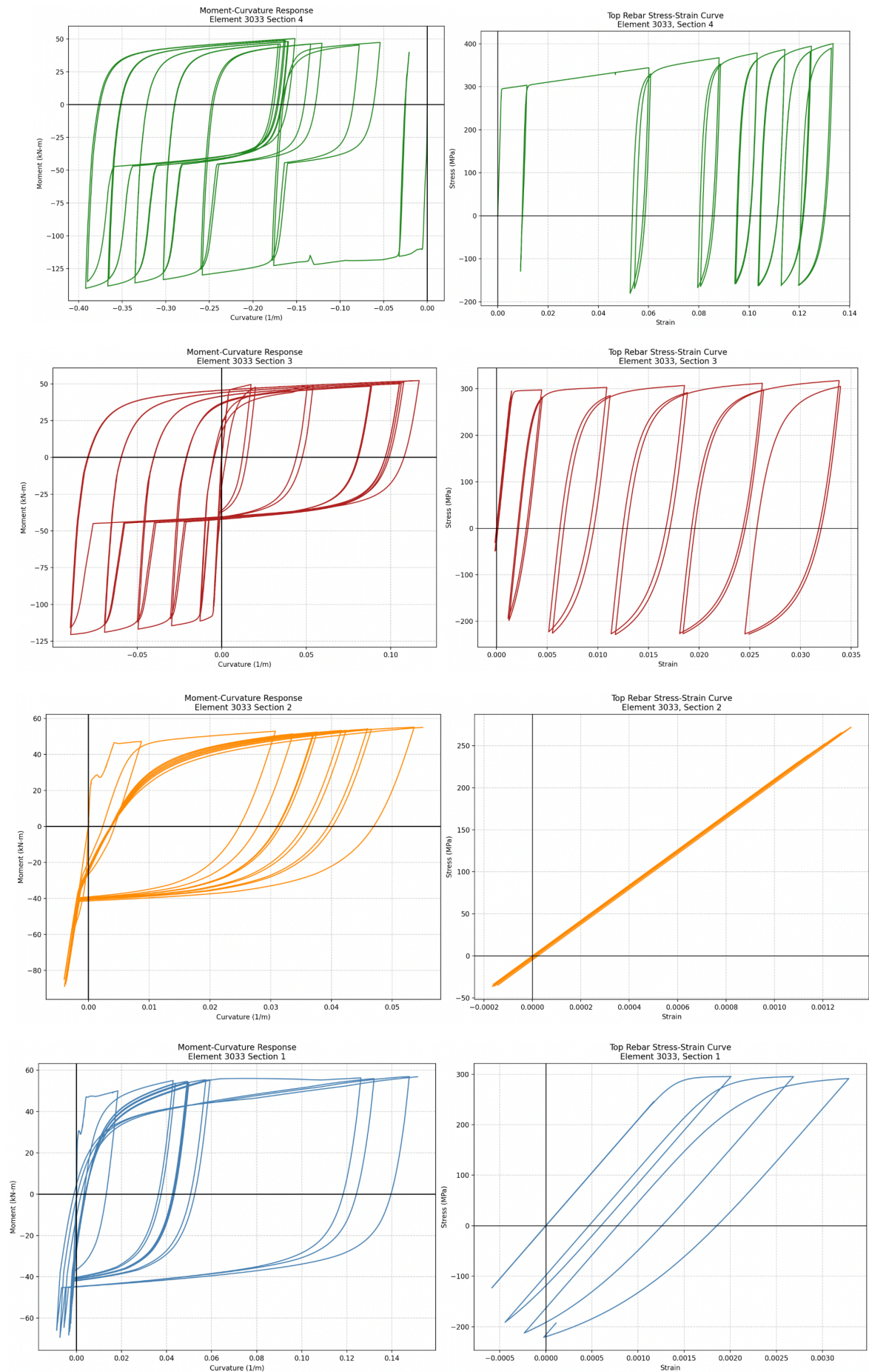
Figure 13. Section Moment-Curvature and Stress-Strain response of corner rebar of Model 0 With Force-based elements
