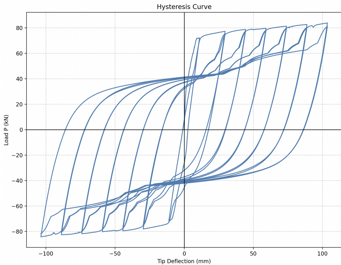
Figure 4. Numerical Response of Model 0
