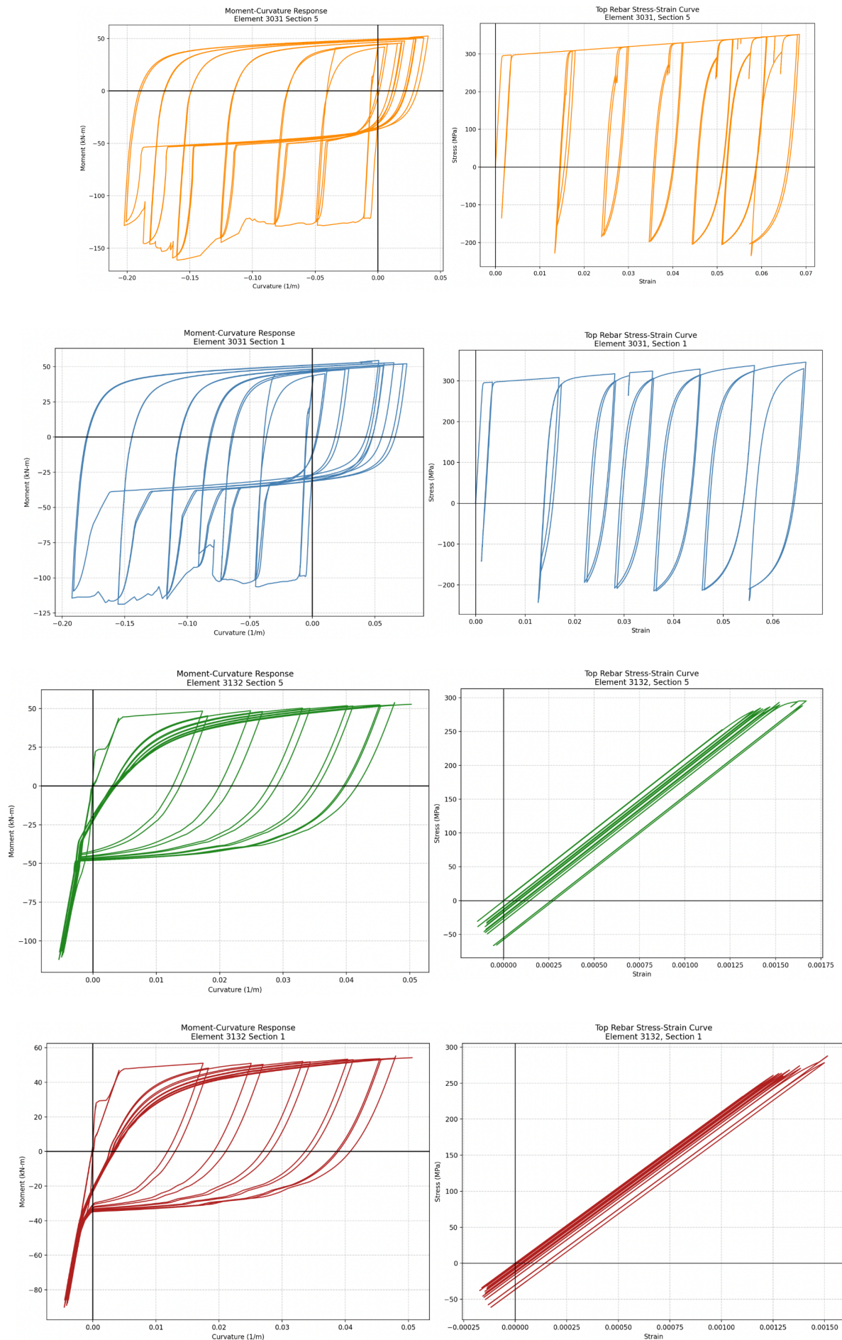
Figure 8. Section Moment-Curvature and Stress-Strain response of corner rebar of Model 0
