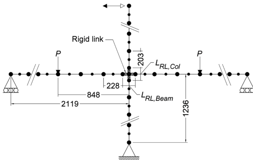
Figure 1. FE modeling
