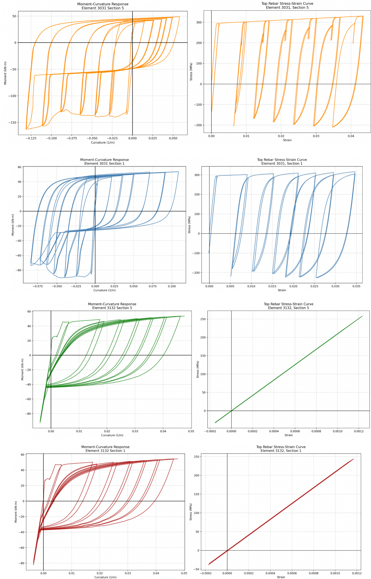
Figure 9. Section Moment-Curvature and Stress-Strain response of corner rebar of With Double Plastic Hinge Length
