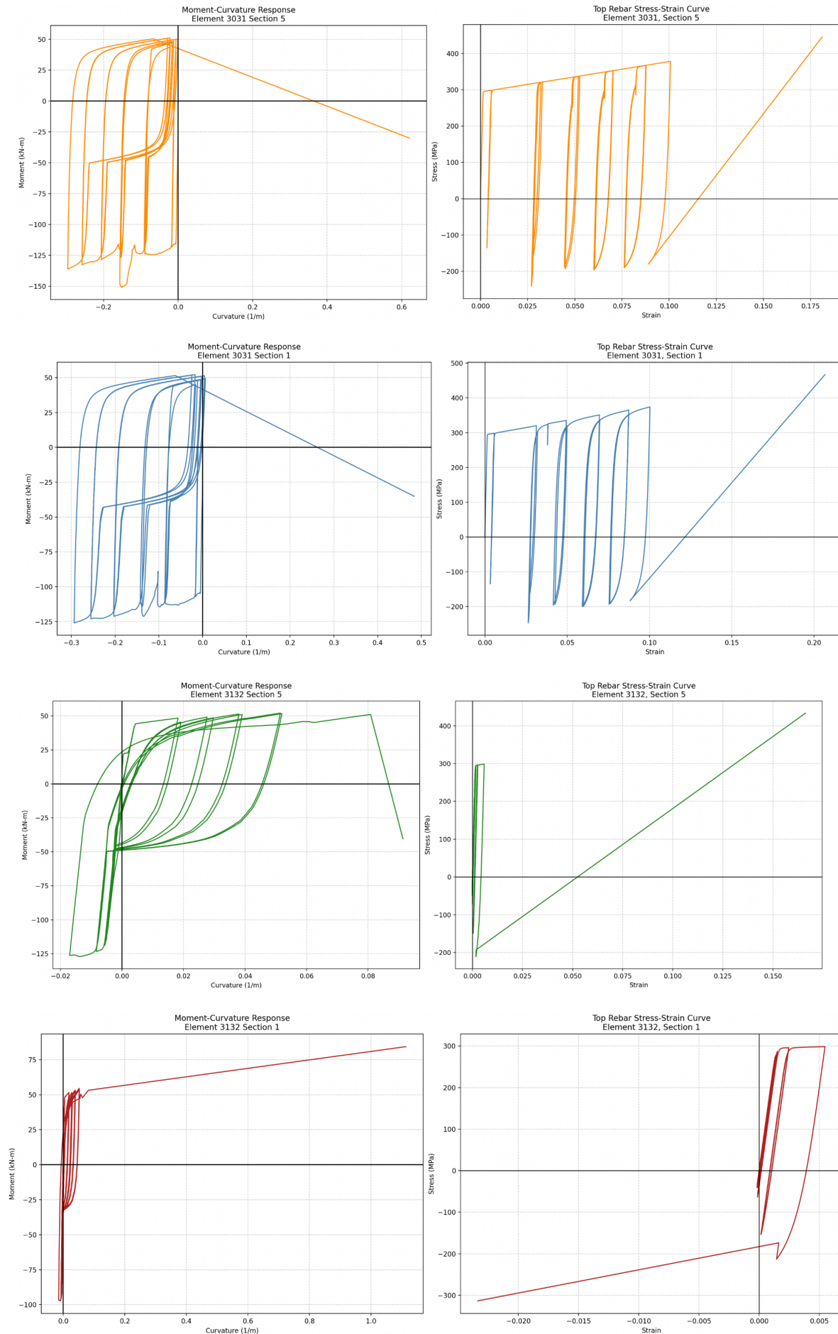
Figure 10. Section Moment-Curvature and Stress-Strain response of corner rebar of With Halved Plastic Hinge Length
