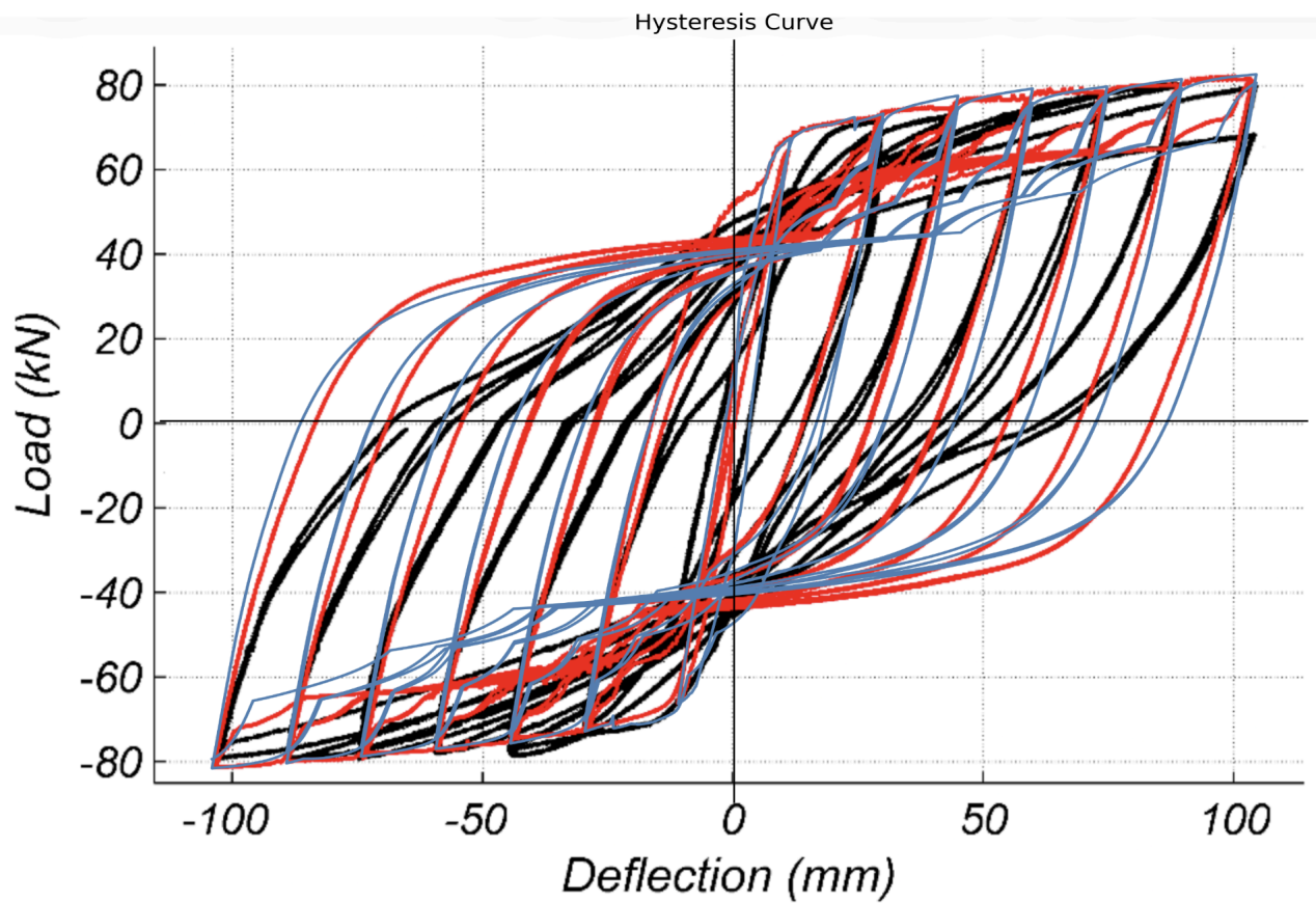
Figure 11. Expected numerical (red), Observed numerical (blue), Experimental (black) correlation of Model 0 With Force-based elements
